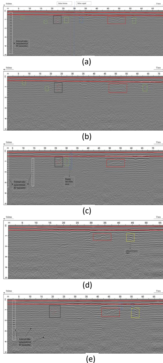
Figure 2. The processed data of line 1 (a) to 5 (e) displayed with hyperbolic response indicating the presence of buried utilities.
