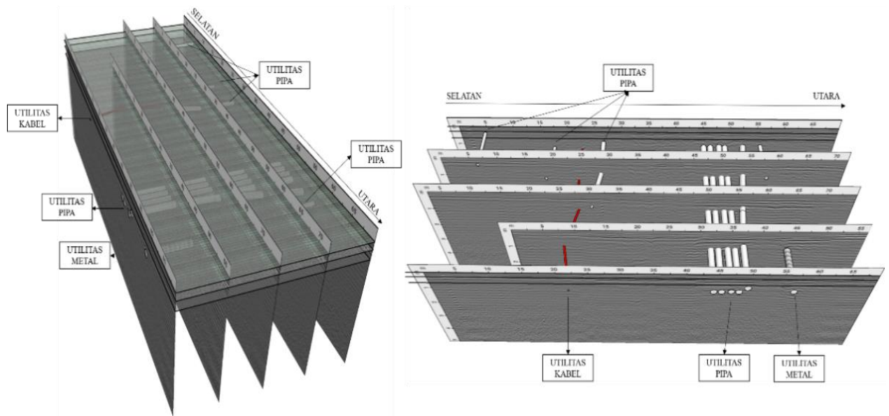
Figure 3. Visualization of GPR data on 5 lines with a depth of \pm 5 m
